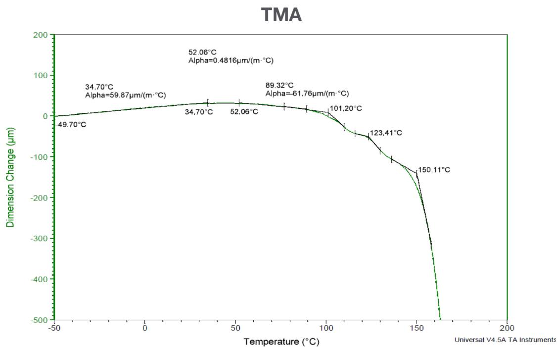
Figure 2. Dimension change data as a function of temperature for the PC-ABS Flat (XY) sample.
