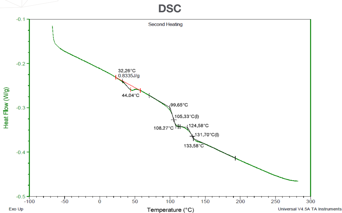
Figure 1. 2nd heating scan DSC data for the PC-ABS Flat (XY) sample.
