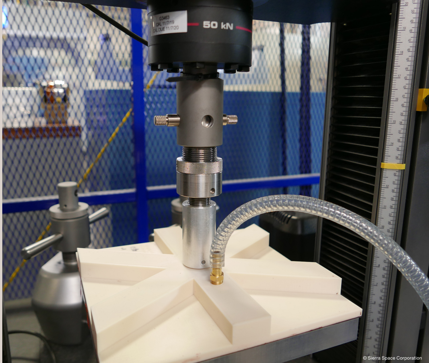
Qualification of the 3D printed chuck.
